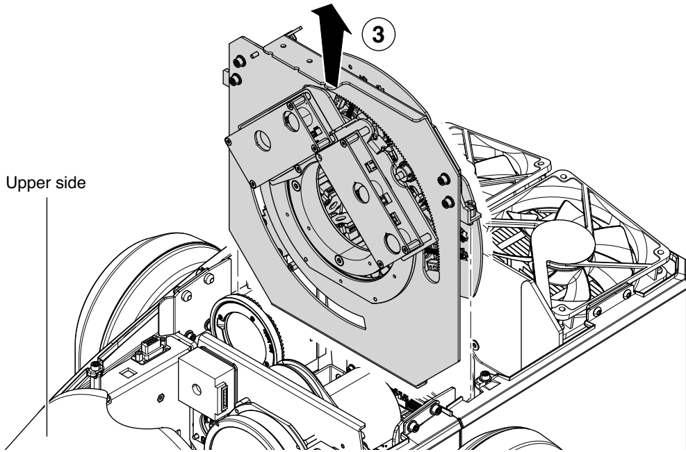
Extraction of the effect modules - Fig. 17.
