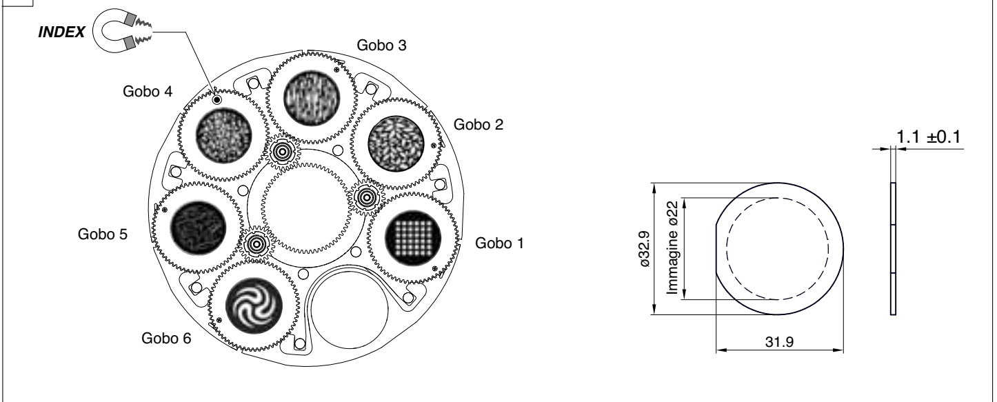
Replacing rotating gobos (max 22 mm image – thickness 1.1 mm) - Fig. 21
