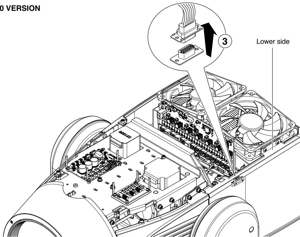
Extraction of the effect modules: Preliminary operations - Fig. 15.
