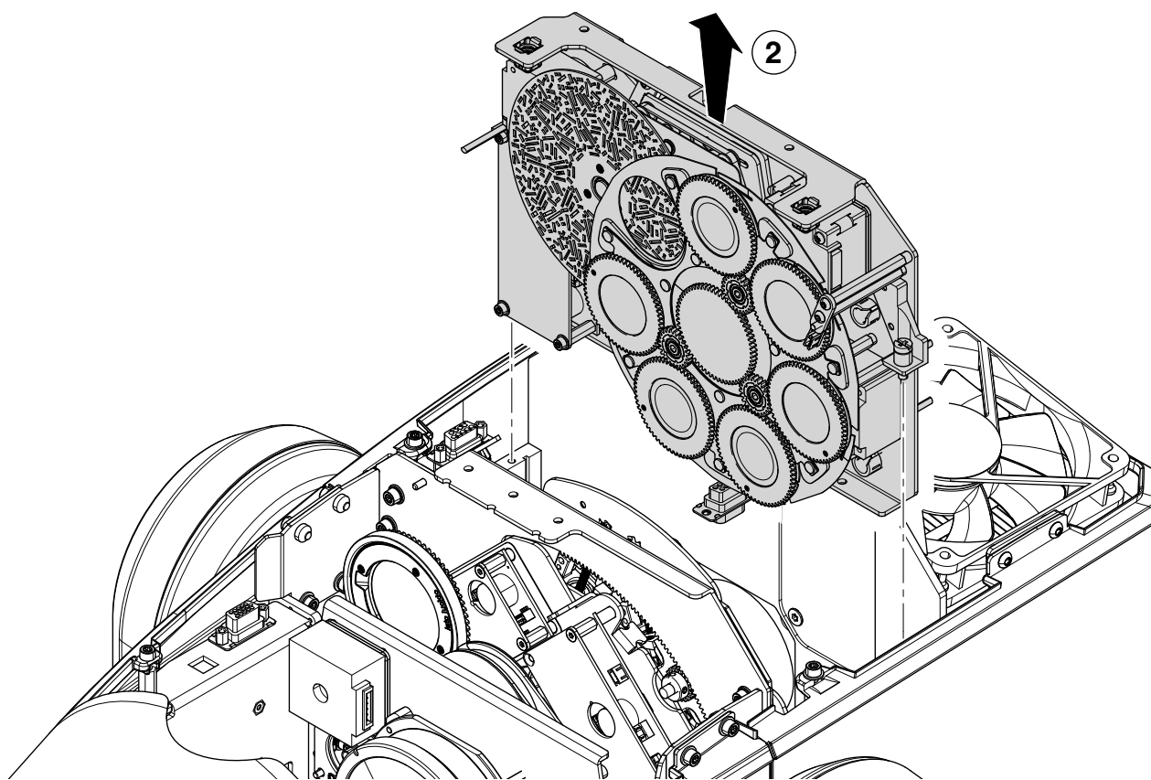
Extraction of the effect modules - Fig. 16.
