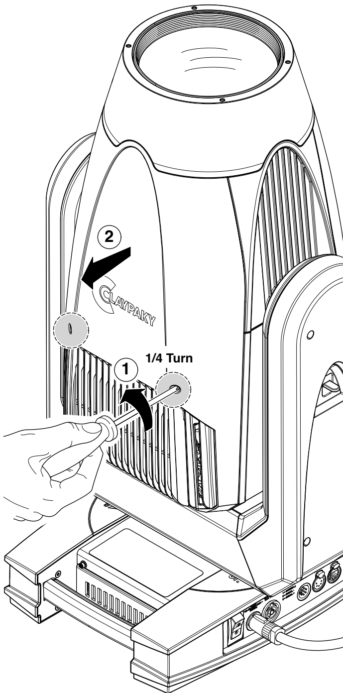
Cleaning of the grids - Fig. 19.
